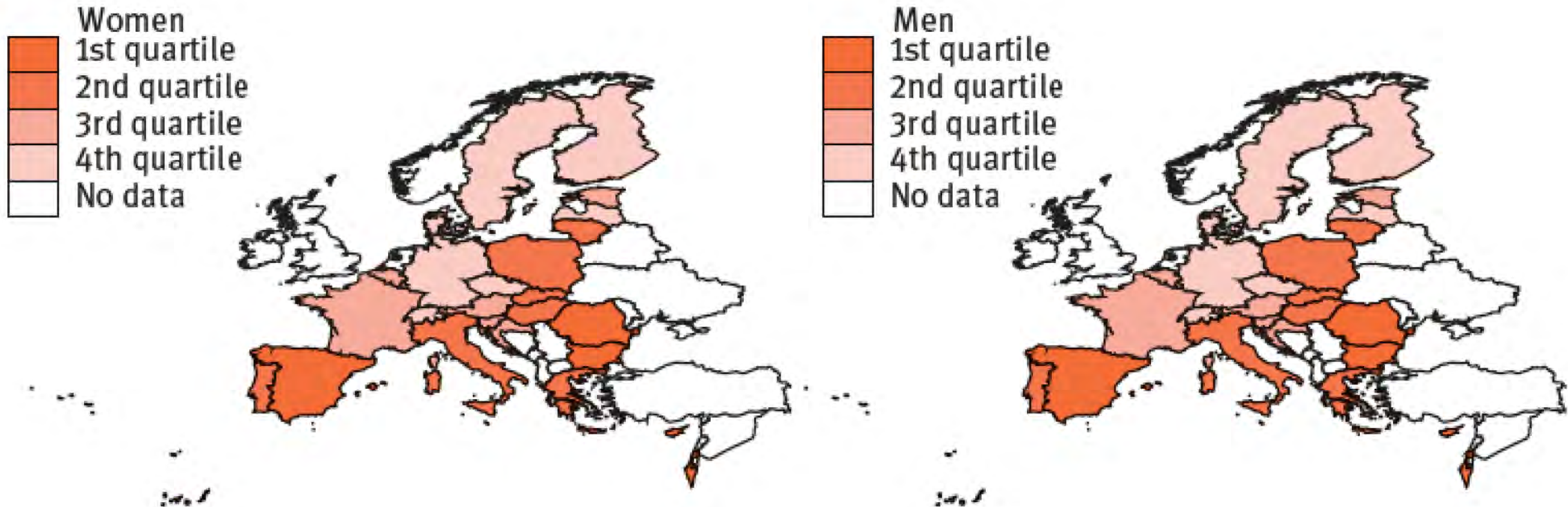
Figure 34.2: Handgrip strength.
